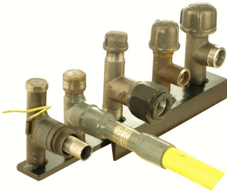
WELD ON TEES
