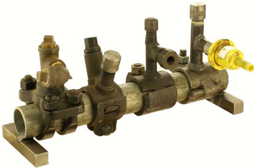
SADDLE TEES ON STEEL PIPE
