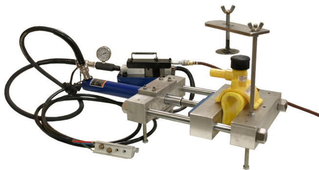
TESTING 6" FUSION TEE
