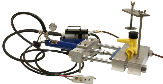
TESTING 2" FUSION TEE
